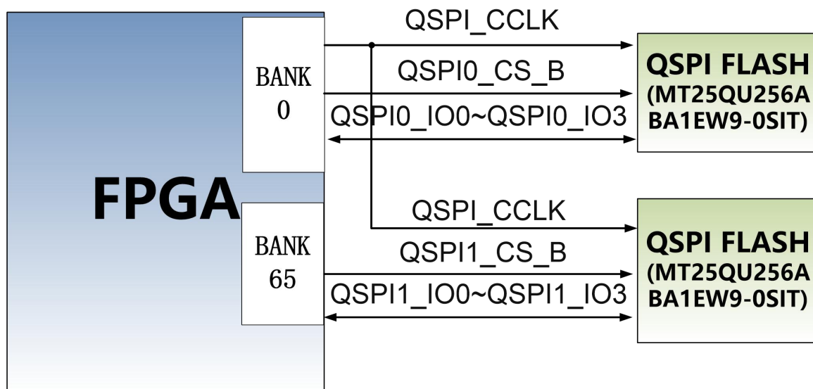
Figure 4-2 QSPI Flash
