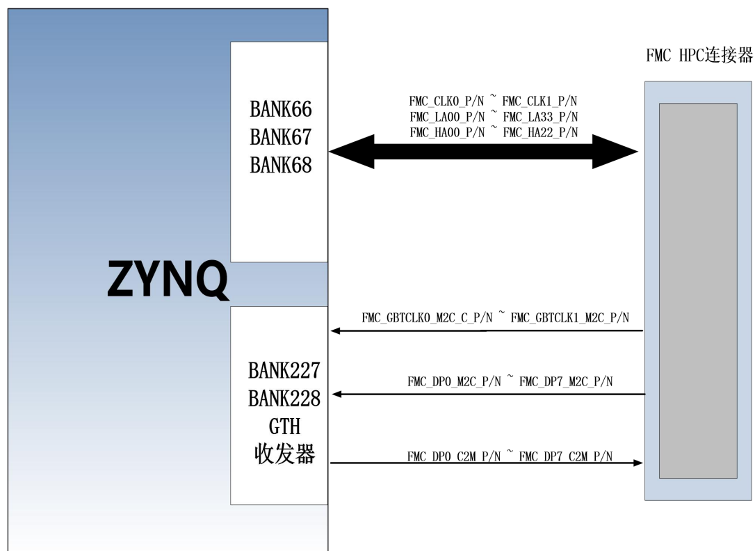
Figure 10-3 HPC FMC3
