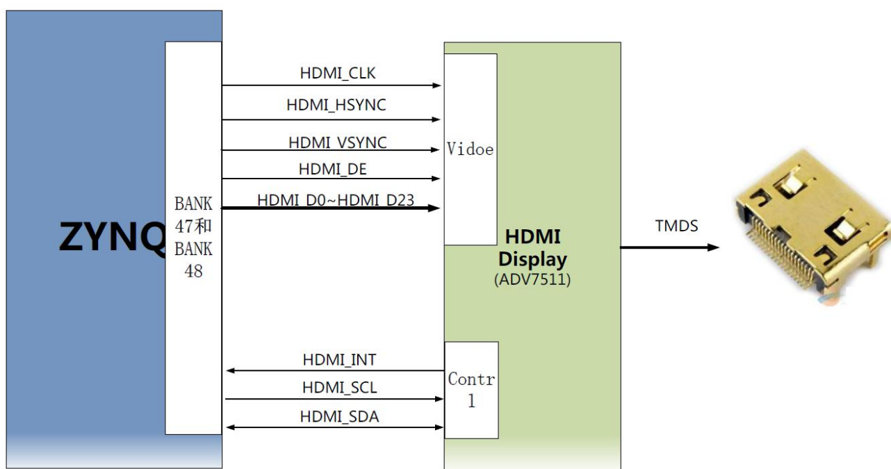
Figure 8-1: HDMI Output Interface Schematic
