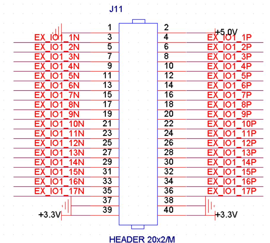
Figure 3-11-1: Expansion header J11 schematic
