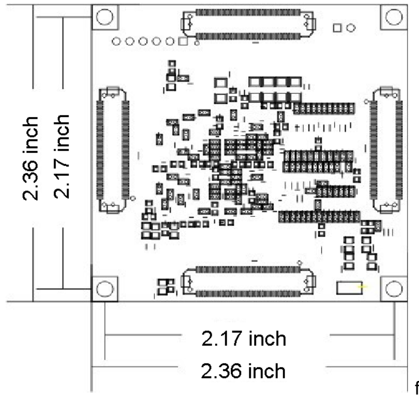
Figure 2-11-2: AC7A035 FPGA Core board (Bottom view)
