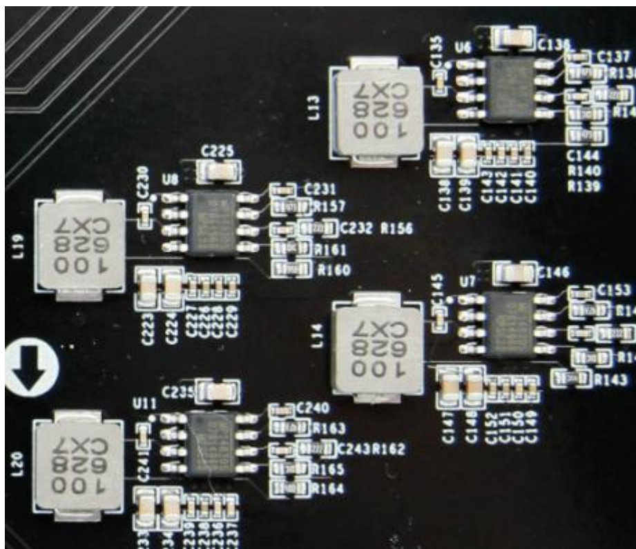
Figure 3-14-3: Power Supply Circuit on the Carrier board
