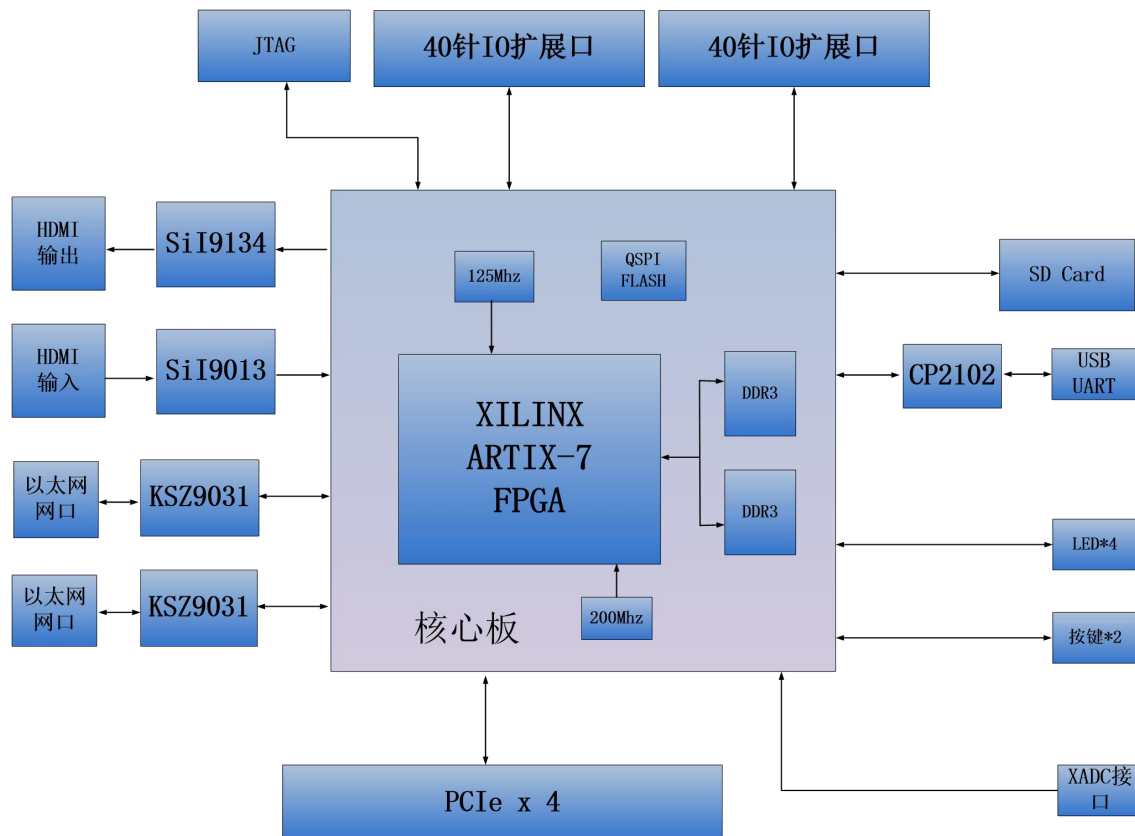
Figure 1-1-1: The Schematic Diagram of the AX7103
