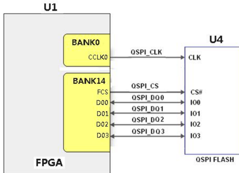
Figure 2-5-1: QSPI Flash Schematic
