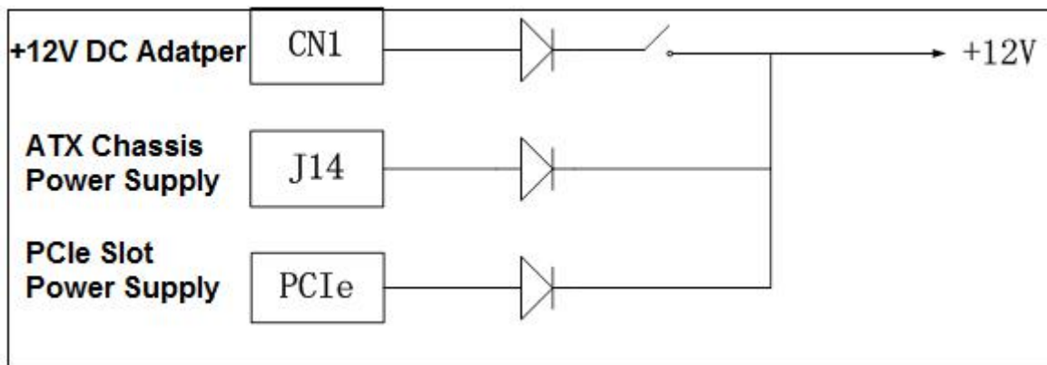
Figure 3-14-1: Power supply method for AX7103 FPGA Board
