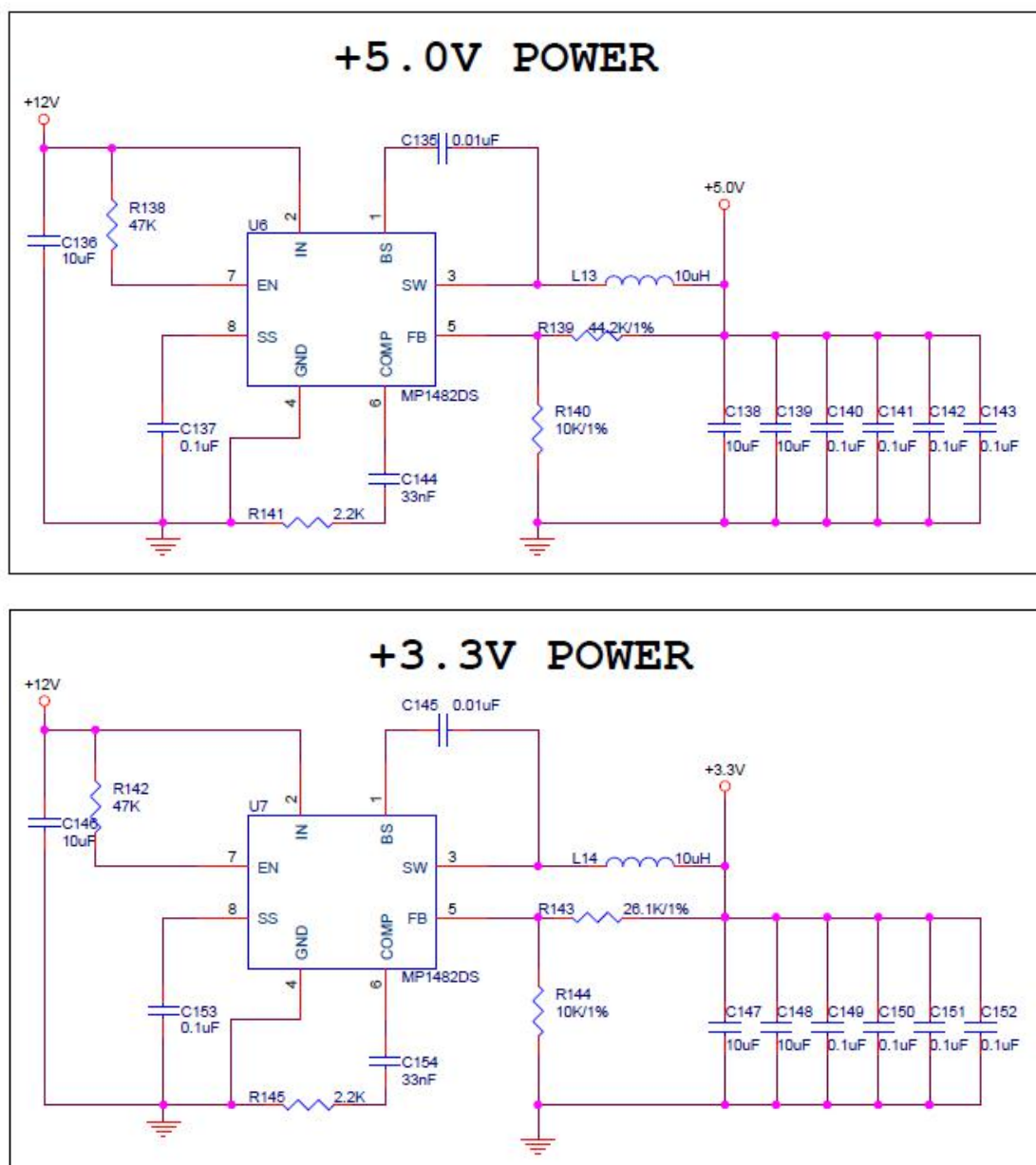
Figure 3-10-1 Power Design Schematic on the Carrier Board
