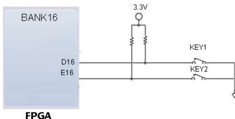
Figure 3-8-1: Key Schematic
