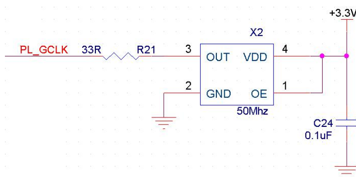
Figure 2-6-3: PL system clock source
