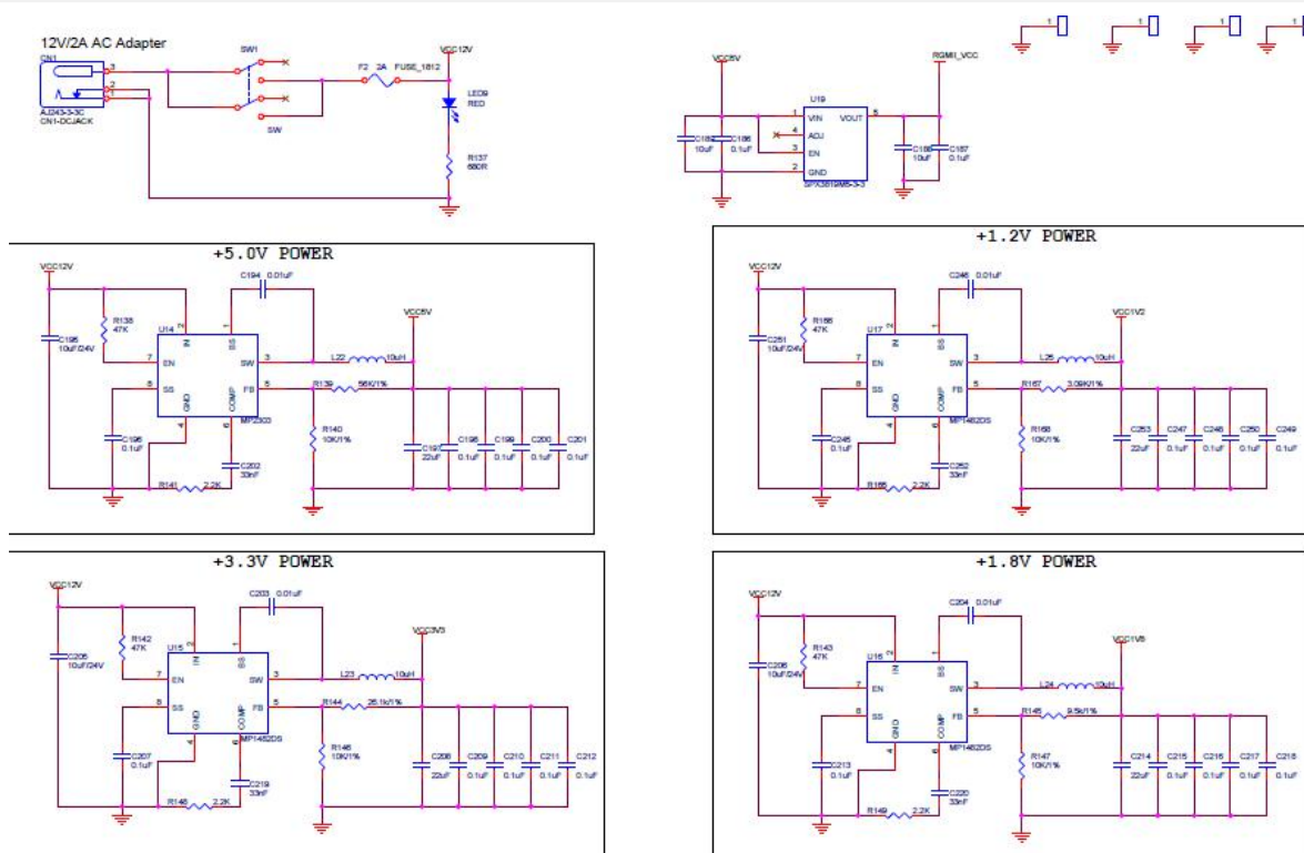
Figure 3-11-1: Power Supply Schematic on the Carrier Board
