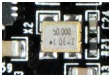
Figure 2-6-4: 50Mhz active crystal oscillator on the Core Board
