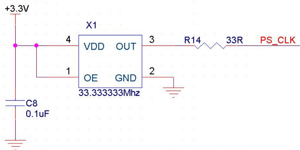
Figure 2-6-1: Active crystal oscillator to the PS section
