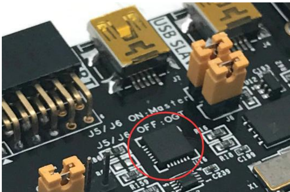
Figure 6-9: CP2102GM chip on the FPGA Board
